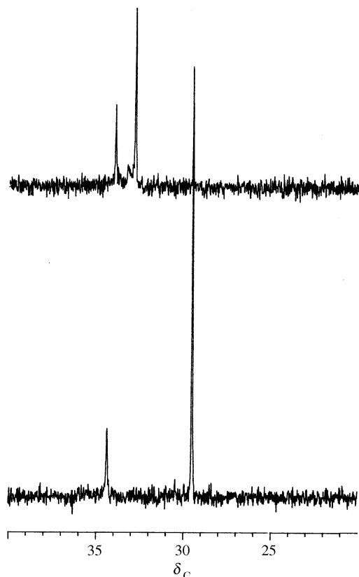
Fig. 3 ^{13}\text{C} NMR spectra of (a) dodecamer 5'-CACCG*ACGGCGC-3' where G* is 2- N -( ^{13}\text{C} )methyl)guanine and (b) duplex formed by 5'-CACCG*ACGGCGC-3' and 3'-GTGGCTGCCGCG-5'. The peak at \delta_{\text{C}} 29.5 is the methyl carbon of acetate used as a reference.
