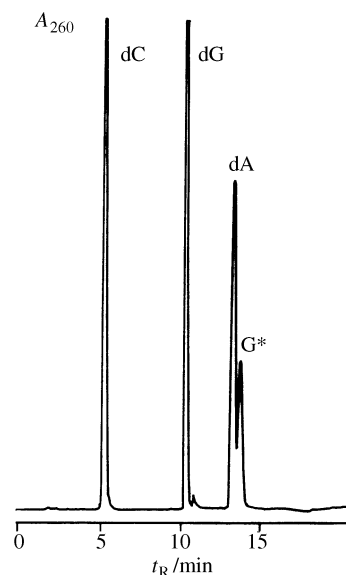
Fig. 2 Enzymic digestion of purified 2- N -([ 13 C]methyl)guanine dodecamer {5'-CACCG*ACGCGC-3' where G* is 2- N -([ 13 C]methyl)guanine}
