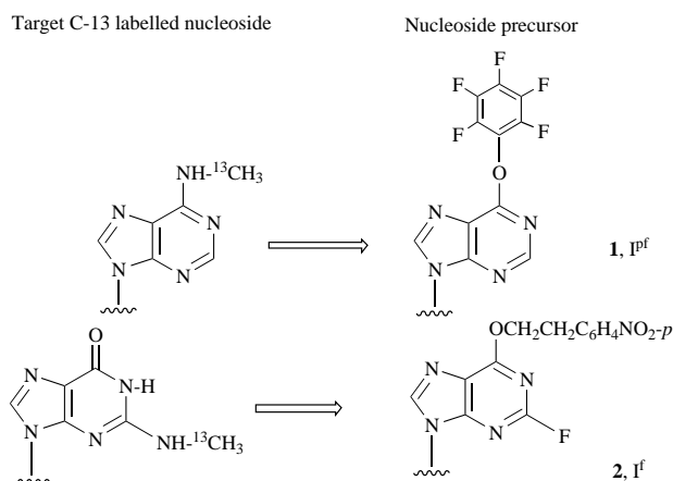
Scheme 1 Nucleoside derivatives used in this work for the preparation of oligonucleotides containing 6- N -([ 13 C]methyl)adenine and 2- N -([ 13 C]methyl)guanine
