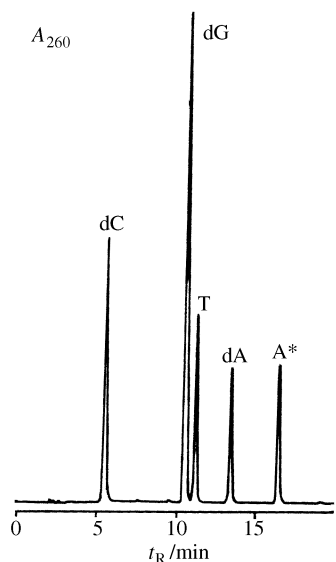
Fig. 1 Enzymic digestion of purified 6- N -([ 13 C]methyl)adenine dodecamer {5'-GCCGAA*TCGCGC-3' where A* is 6- N -([ 13 C]methyl)adenine}
